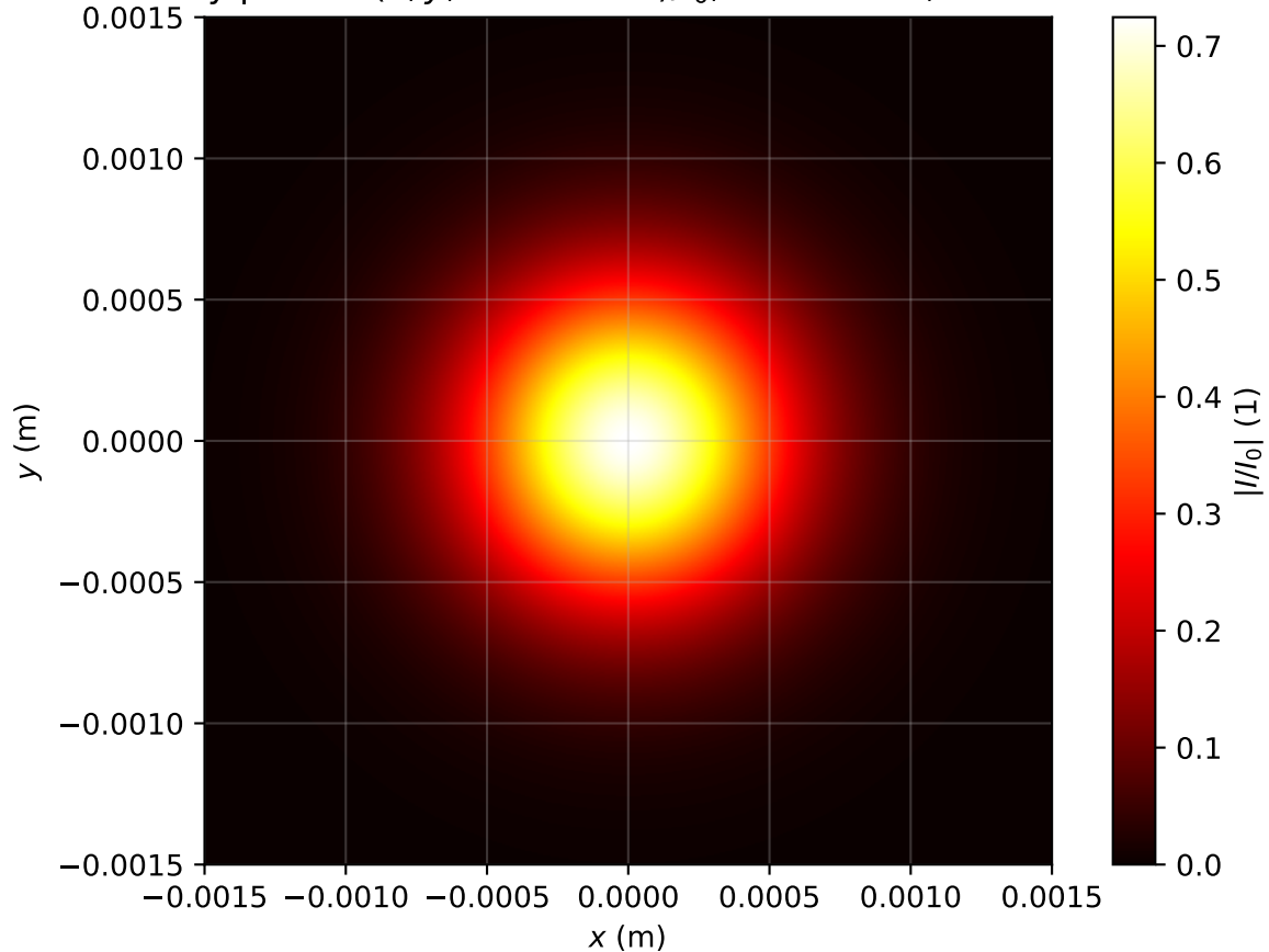
Intensity profile I(x, y, z = 1.751m)/I_0 , Pin=0.3Pcr, artificial time
